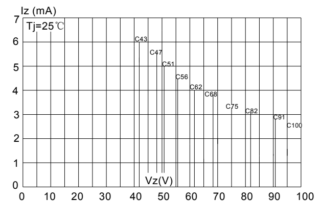
Fig.4 Zener breakdown characteristics
